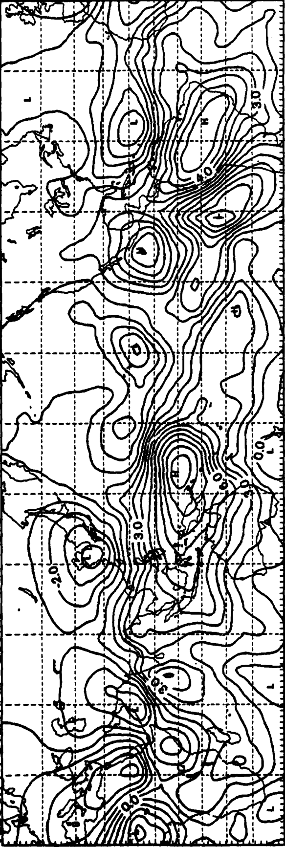
VELOCITY POTENTIAL 200MB JAN 1975
